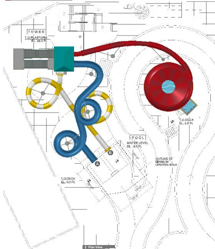
1 Plan View
