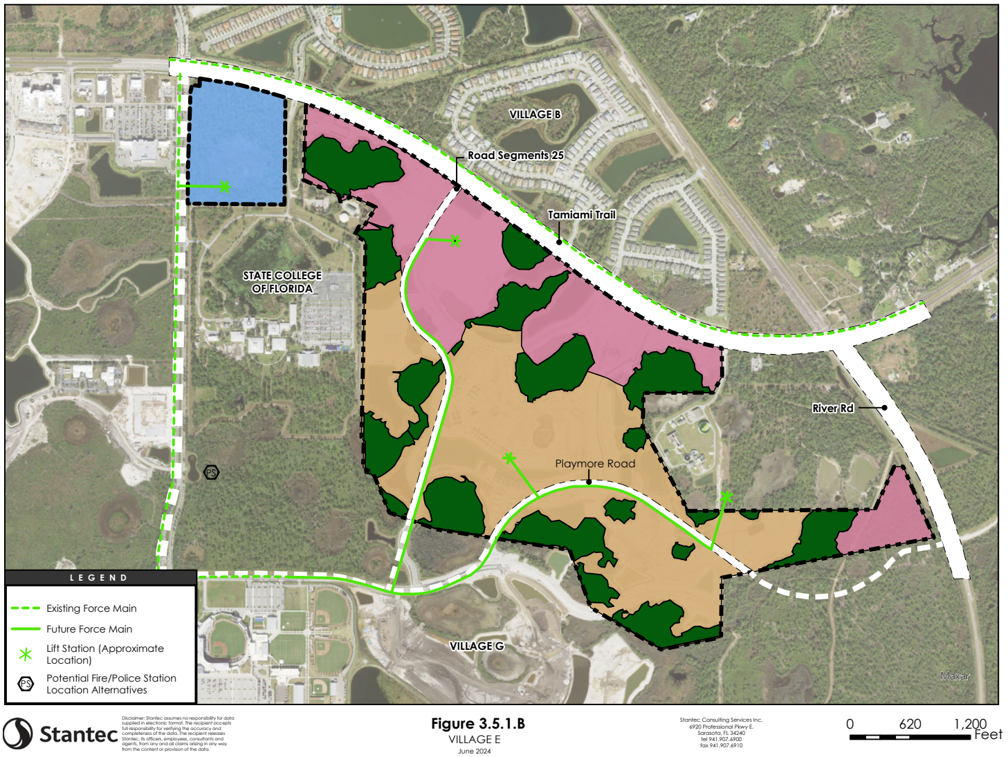
Figure 3.5.1.B Wastewater Systems Plan
