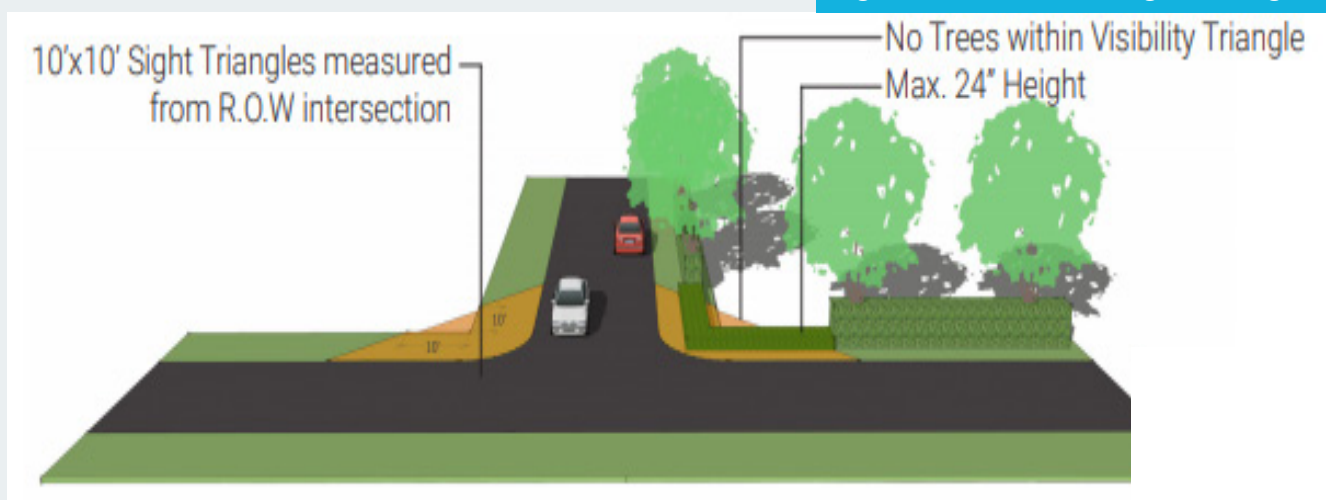
Figure 27 – 10' X 10' Sight Triangles
