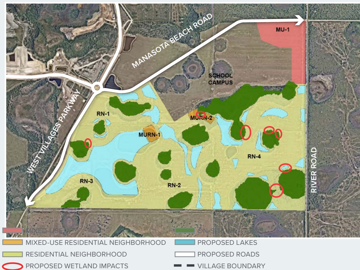
Figure 15 – Wetland Impact Plan
