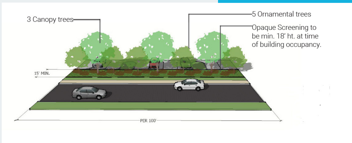
Figure 26 – Trees and Screening
