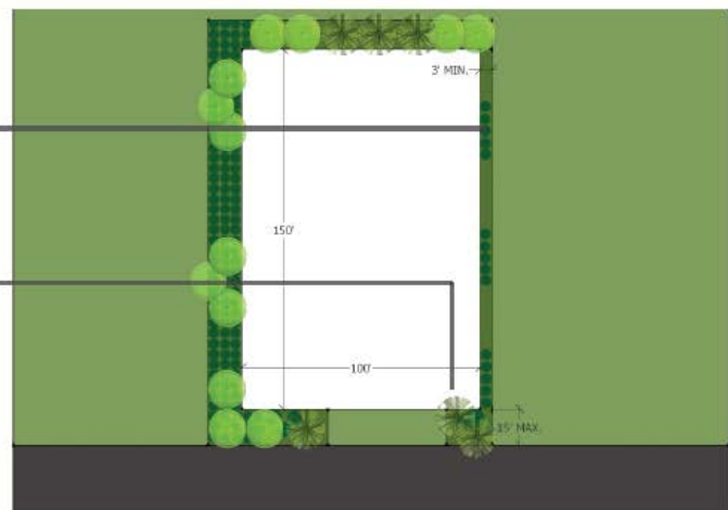
Figure 33 – Landscape Buffer Example 2
