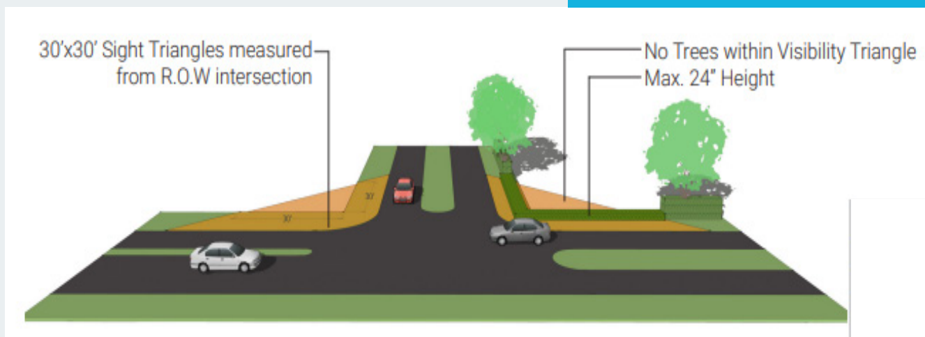
Figure 28 – 30' X 30' Sight Triangles
